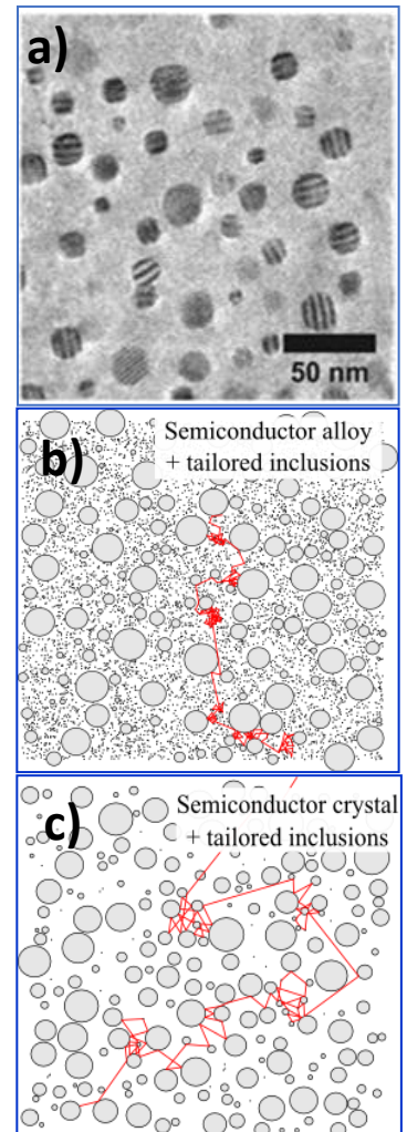
Figure 1 : a) TEM image of GeMn thin layers including nano-inclusions. b, c) sketches of phonons transport in GeSnMn vs GeMn samples showing the expected influence of superdiffusivity.
